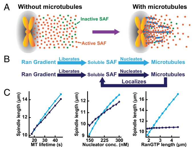
Fig. 4. The localization of SAFs by spindle microtubules implies a feedback based on spatial localization. (A) A cartoon showing the distribution of activated (orange circles) and inactivated cargoes (green circles) when microtubules are absent (Left) and when microtubules are present (Right) in a mitotic cell. (B) In the absence of microtubule interactions, the Ran pathway would be linear (Top, cyan). The interaction between SAFs and microtubules leads to a feedback based on spatial localization because SAFs that nucleate microtubules localize where microtubules are present (Bottom, dark blue). (C) (Left) Simulated spindle length as a function of microtubule lifetime without (cyan squares) and with (dark-blue squares) the interaction of the SAF with microtubule. (Middle) Simulated spindle length as a function of nucleator concentration without (cyan diamonds) and with (dark-blue diamonds) the interaction of the SAF with the microtubule. (Right) Simulated spindle length as a function of the length of the RanGTP gradient without (cyan circles) and with (dark-blue circles) the interaction of the SAF with the microtubule.
